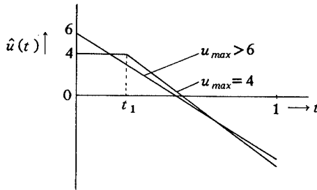
Solution of Example 1 for u_{max} > 6 and u_{max} = 4 .
